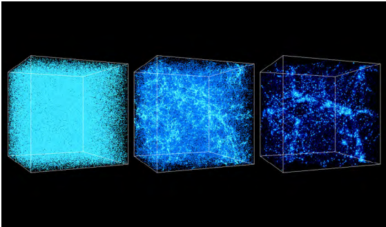
Simulation of the formation of clusters and large-scale filaments in the \Lambda CDM model with dark energy, from z \approx 30 (l), to z \approx 5 (m), to present (r); box dimension = 43 million parsecs. (A. Kravtsov and A. Klypin)
