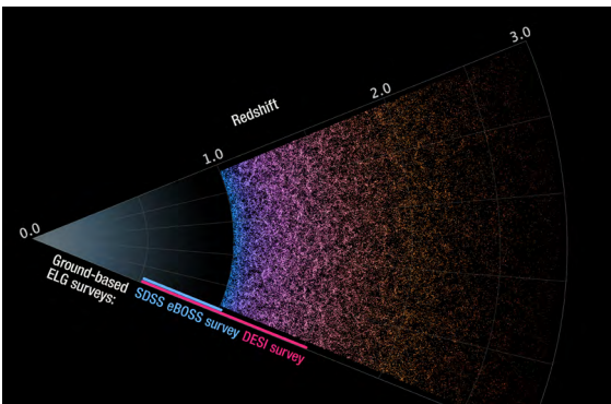
Visualization of simulated Roman emission-line galaxy distribution data used to measure BAO and RSD. The wedge shown covers an RA sweep of 45^\circ with a DEC thickness of 1^\circ , and includes more than 215,000 galaxies. (Data provided by Z. Zhai and Y. Wang, Caltech/IPAC and A. Benson, Carnegie Observatories, Visualization by J. DePasquale, STScI)
