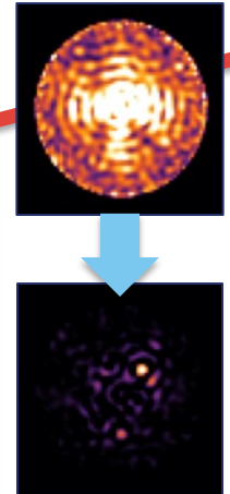
Data Post-Processing
