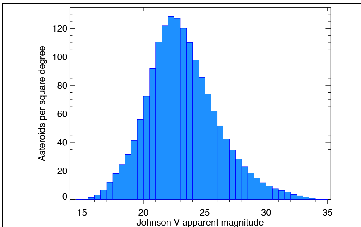
Figure 1: Frequency of main belt asteroids (MBAs) between 10 m and 27 km in diameter per square degree as a function of apparent magnitude in the Johnson V filter. The peak frequency is between 22.0 and 22.5 mags. These results are representative of the entire population of minor bodies in the solar system, not just MBAs, due to the much smaller number of other (detectable) minor bodies and the observation bias towards larger targets at larger heliocentric distances. Assuming a uniform distribution of objects, hundreds of minor bodies should be present in each square degree of sky near the plane of the ecliptic.
